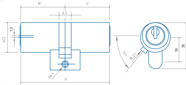
SEA 3 / SEA 23 Cylinder
