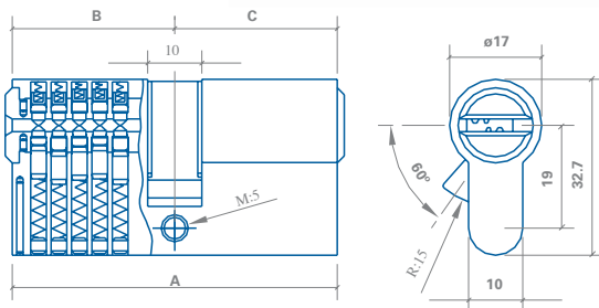
DS-10 Switch cylinder
