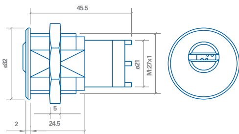
DS-10 Switch cylinder
