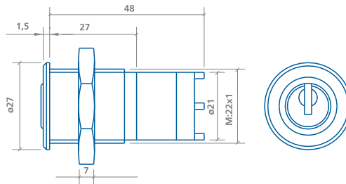
SEA 3 / SEA 23 Switch cylinder
