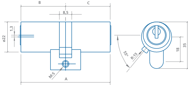
SEA 3 / SEA 23 Cylinder
