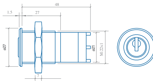
SEA 3 / SEA 23 Switch cylinder
