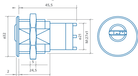
DS-15 Switch cylinder
